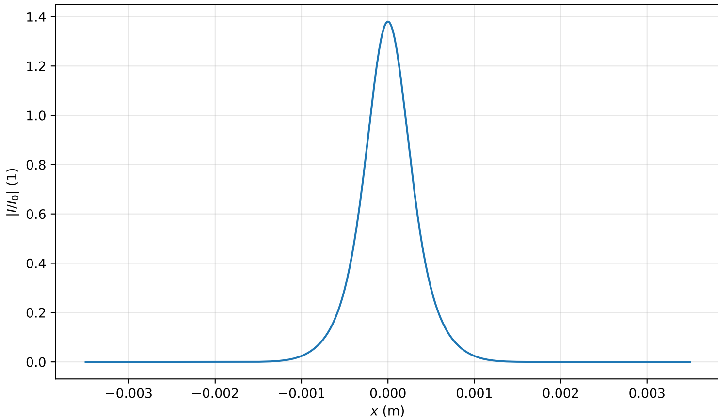
Intensity profile I(x, y = 0, z = 0.955m)/I_0 , P_{in}=0.9P_{cr} , artificial time
